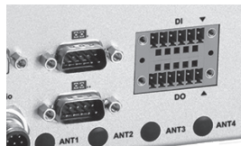
Isolated RS-232/422/485 and DIO ports
