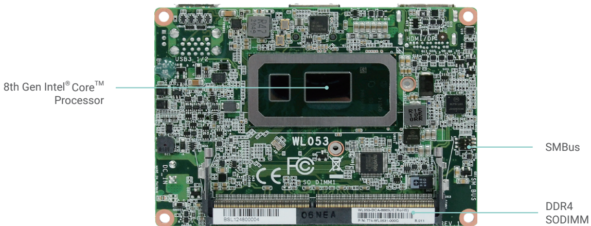
Bottom View
