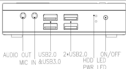
Rear Panel External I/O
