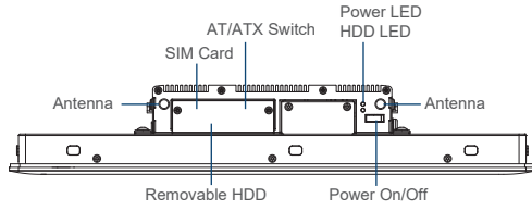
Front I/O
