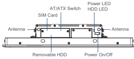
Front I/O
