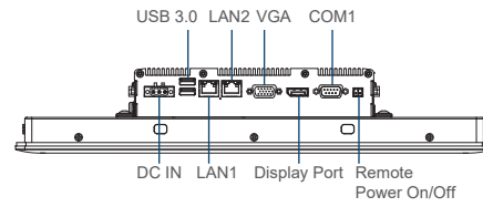
Rear I/O
