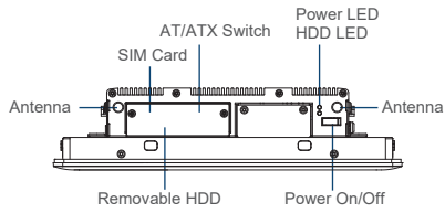
Front I/O
