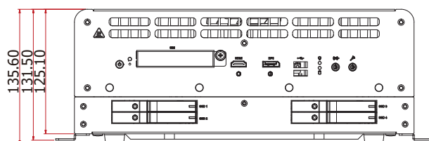
Rear View
