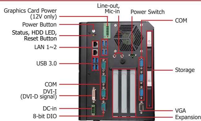
Rear View EC532-KD-AI6881
