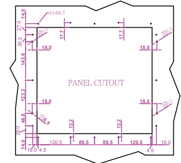
CUT OUT DIMENSION
