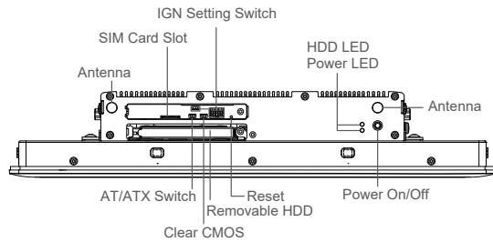
Front I/O
