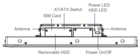
Front I/O
