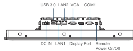
Rear I/O
