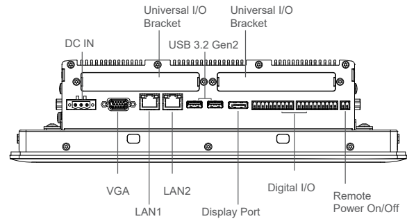
Rear I/O
