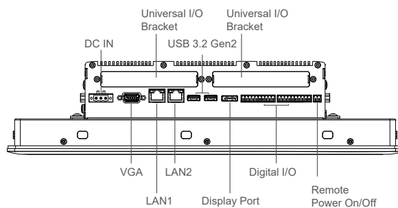
Rear I/O
