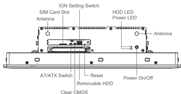
Front I/O
