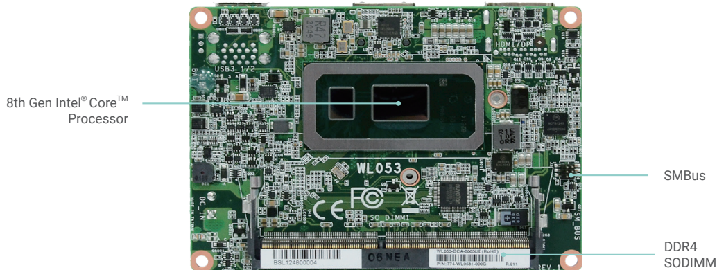
Bottom View
