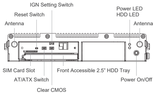
Front I/O
