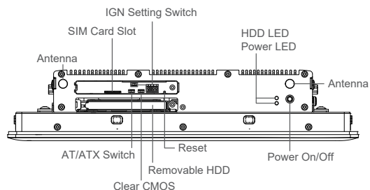
Front I/O
