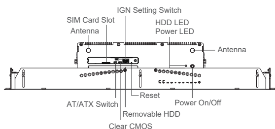
Front I/O
