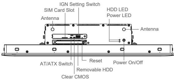
Front I/O
