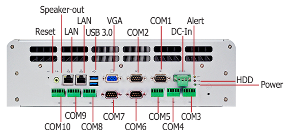
EC300-CRA060 Rear View
