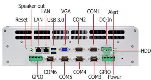
EC300-CR6G60 Rear View
