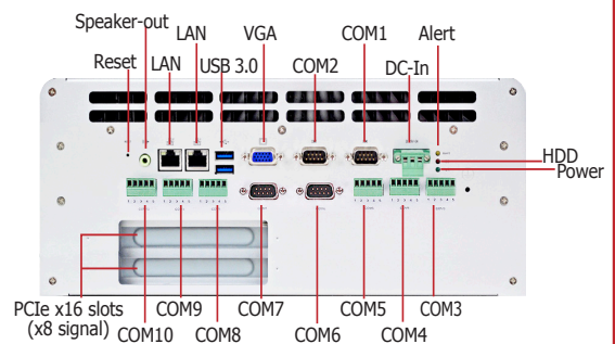
EC322-CRA060 Rear View
