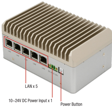
BOXER-8250AI-A4 Front View
