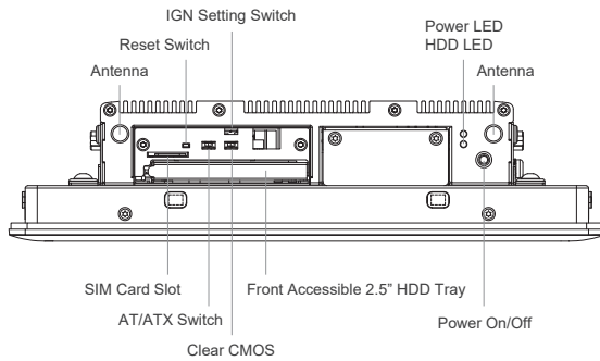
Front I/O
