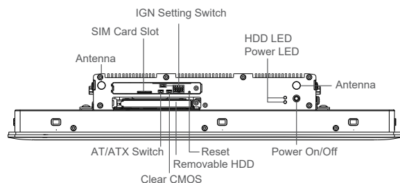
Front I/O
