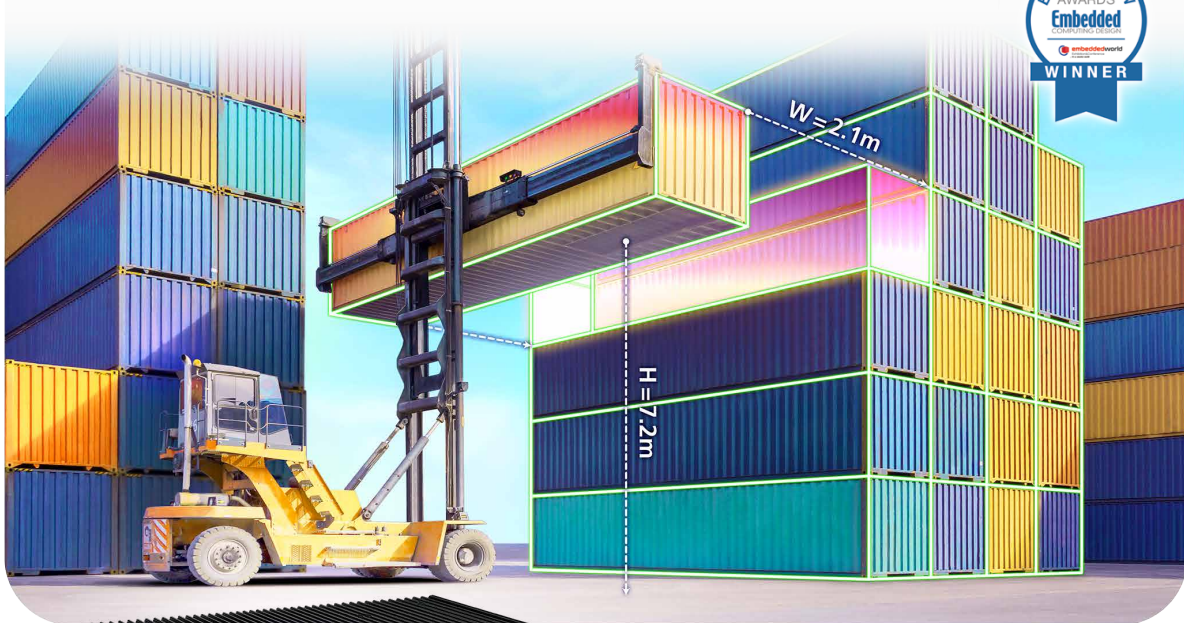
^ AI-powered Cargo
