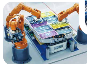
▼ Machine Vision
