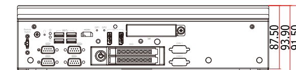
Rear View
