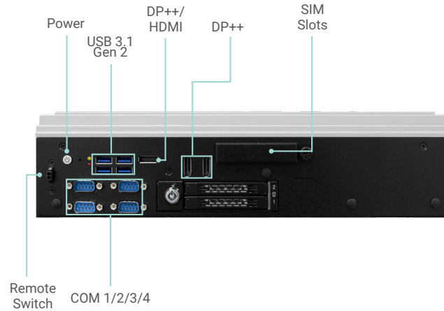
Rear View
