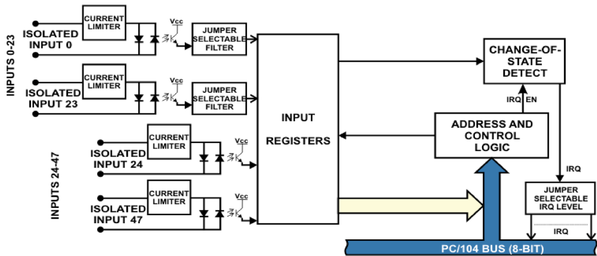
BLOCK DIAGRAM
