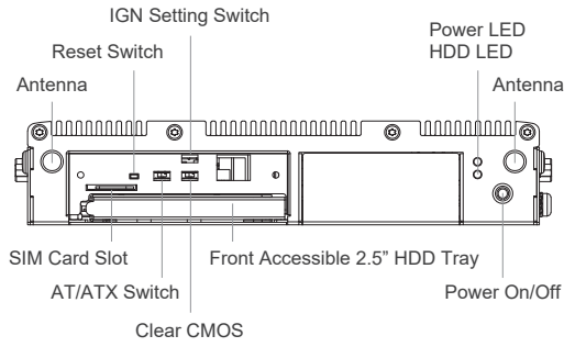
Front I/O
