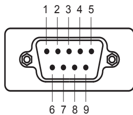
DB-9 Male
