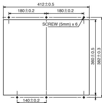
Panel aperture dimensions
