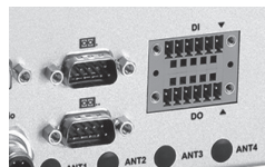
Isolated RS-232/422/485 and DIO ports
