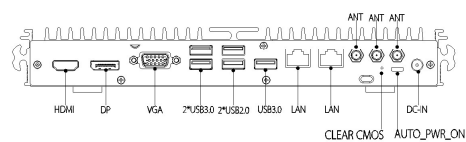
Rear Panel External I/O
