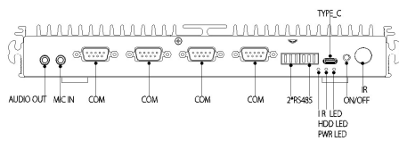
Front Panel External I/O
