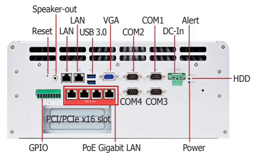
EC320/321-CR4866 Rear View
