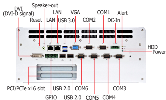
EC320/321-CR6881 Rear View
