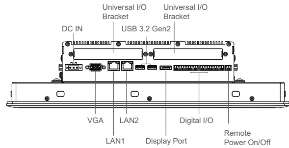
Rear I/O
