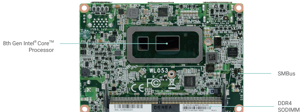
Bottom View
