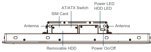
Front I/O
