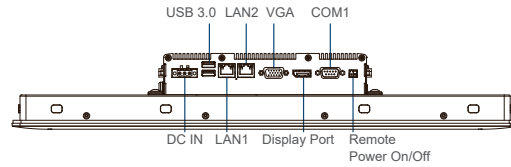
Rear I/O
