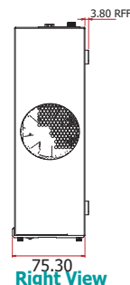
Right View
