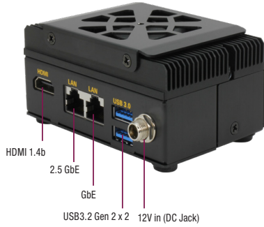
With Heatsink
