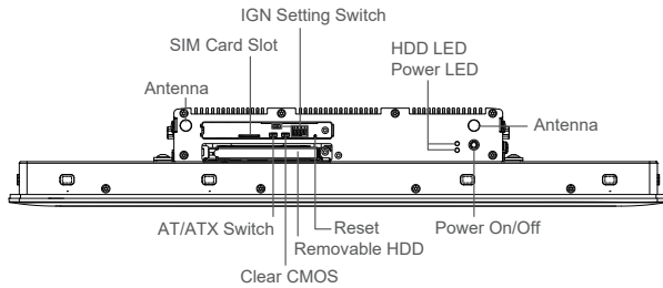
Front I/O
