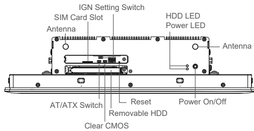
Front I/O
