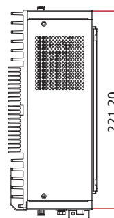
Right View
