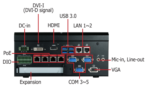
Rear View
