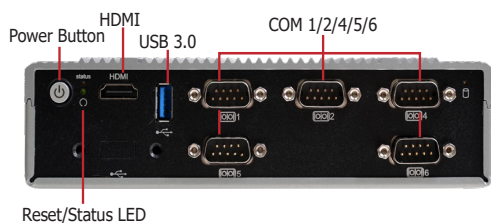
Front View(BT6051)
