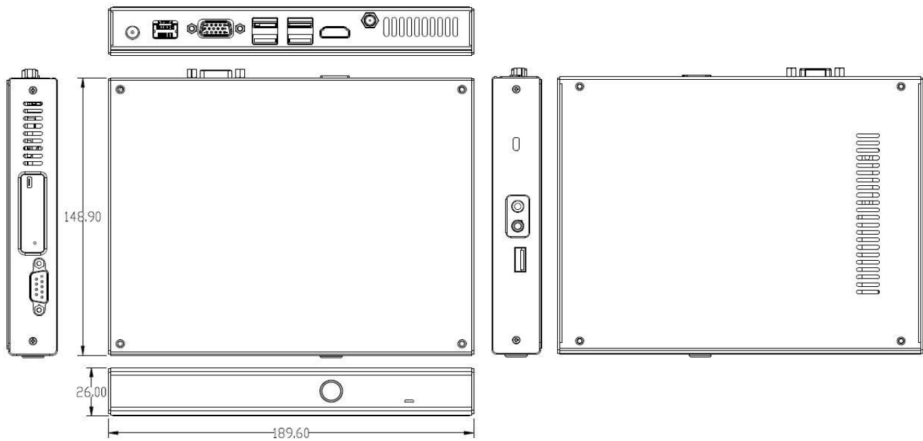
Front Panel External I/O
