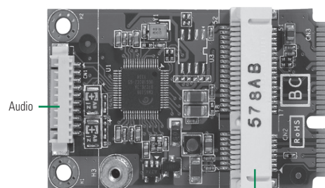
Full-size PCI Express Mini Card (PCIe only)
