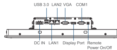
Rear I/O
