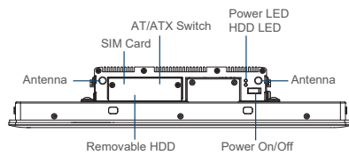
Front I/O
