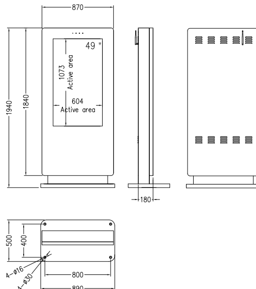
Note: The Ø30 holes are for access, we recommend using M10 anchor bolts that will fit into the Ø16 holes.
