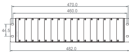
Panel View
