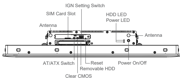
Front I/O
