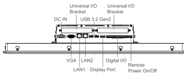
Rear I/O
