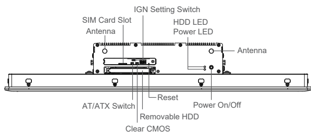
Front I/O
