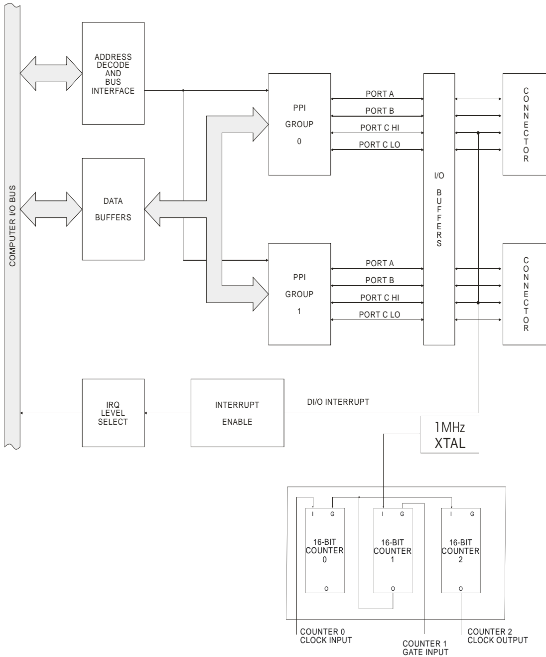
Figure 1-1: Block Diagram
