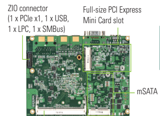
DDR3L SO-DIMM ▲ Rear view
